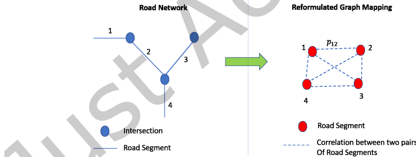
Fig. 3. Problem reformulation to graph problem.
