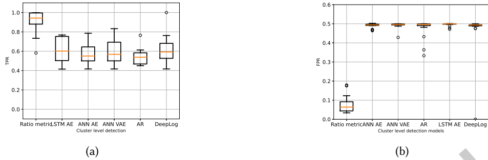
Fig. 13. Cluster level detection with various methods: (a) True positive rates and (b) False positive rates.
