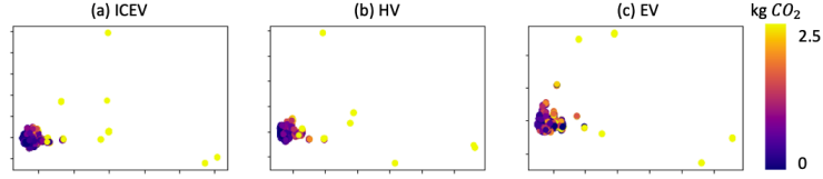
Fig. 7: t-SNE on raw input features for each data sample from the source domain. t-SNE parameters: number of components=2, perplexity=10, initialization=PCA, number of samples=860 (2% of dataset)
