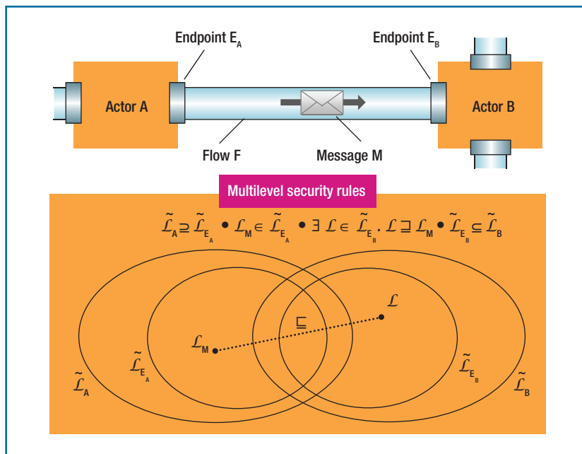
FIGURE 2. Transfer of a message via secure transport. The message goes through a flow that connects an endpoint of the sending actor to an endpoint of the receiving actor. The rules on labels and label sets of actors, endpoints, and messages, guarantee the satisfaction of the Multilevel Security (MLS) policy. The MLS rules are illustrated using Venn diagrams.
