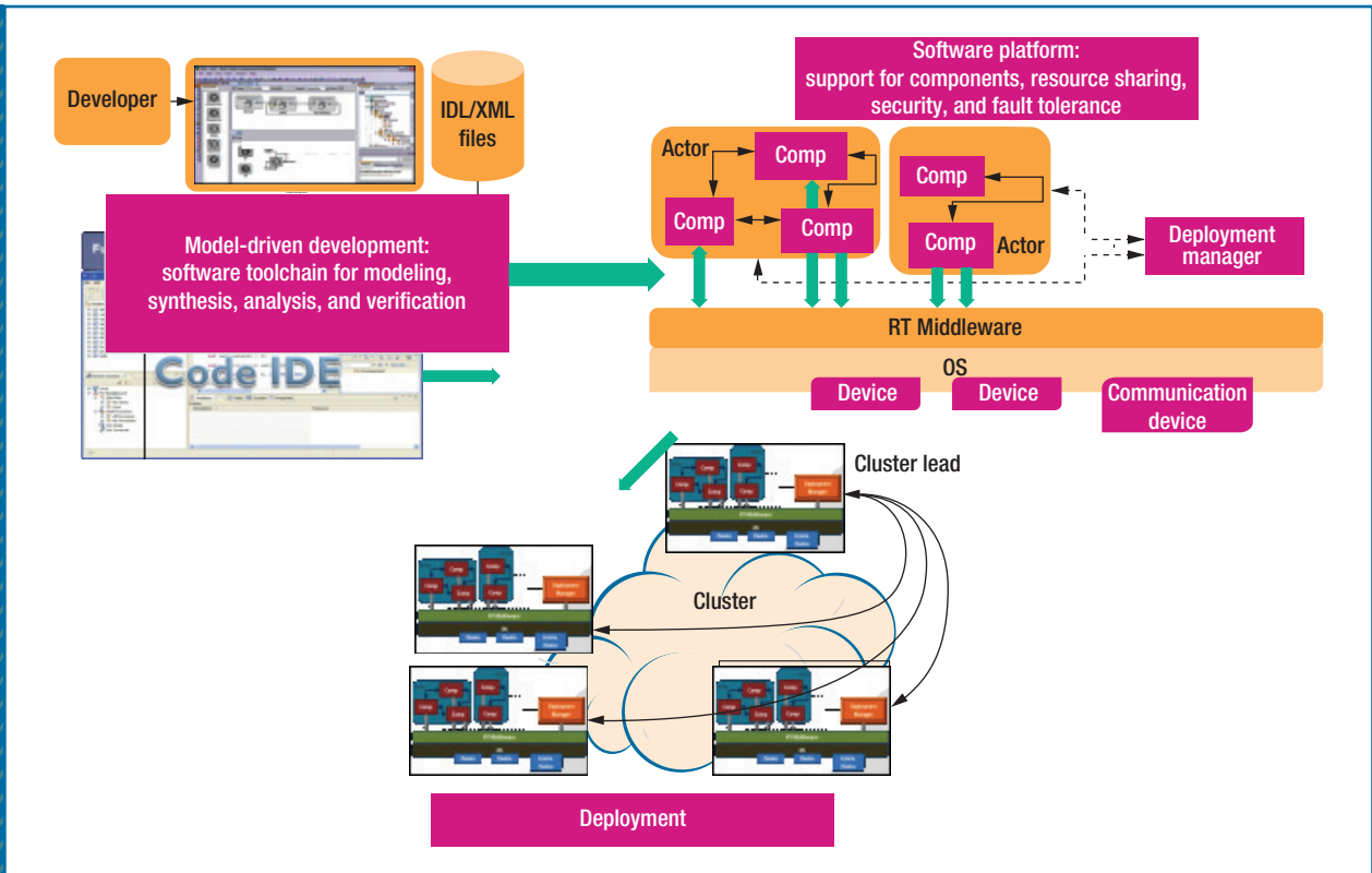
FIGURE 1. DREMS architecture. The top-right portion shows the internals of one node.
