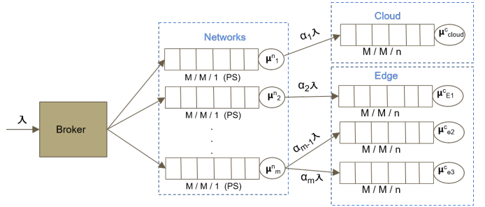
Fig. 3: Diagram of the Workload Simulation Model
