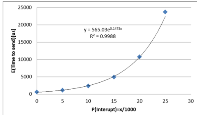
Fig. 2: The expected time to send a message vs. the probability of interruption by uncontrolled external sources
