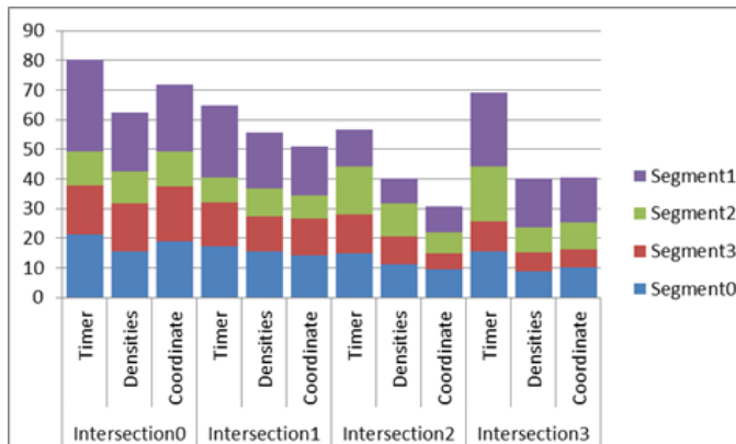
Fig. 6: Compare densities at each intersection using the various controllers
