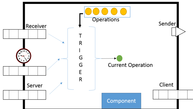
Fig. 1: RIAPS Component Model
