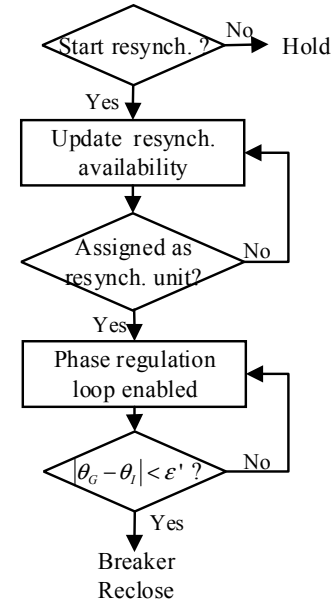
Figure 5. Resynchronization Workflow
